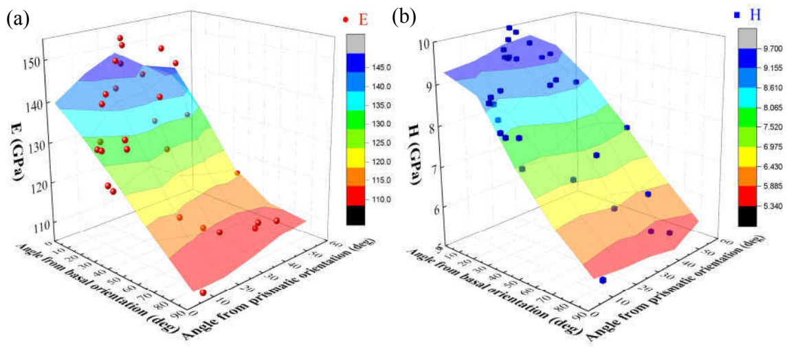
Fig. 8. Experimentally derived mechanical properties of the LATP as a function of the corresponding angle: (a) elastic modulus and (b) hardness, here the colorful surface map is the guide for the eye to see the dependency of mechanical properties on rotation angle.
